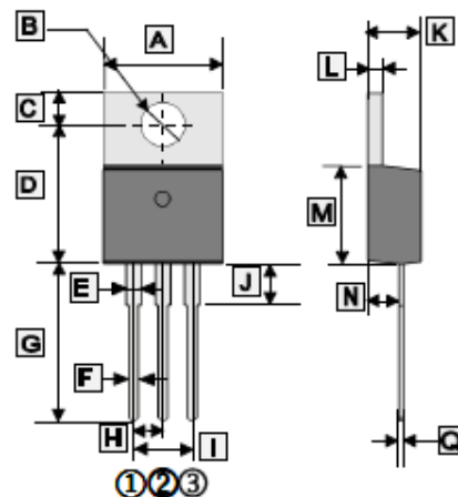
TO-220J
