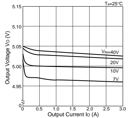
Load Regulation(SI-8050S)
