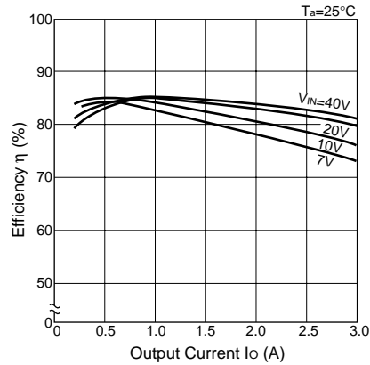
Efficiency Characteristics(SI-8050S)
