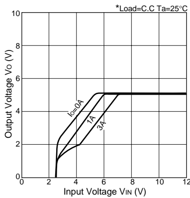
Rise Characteristics(SI-8050S)
