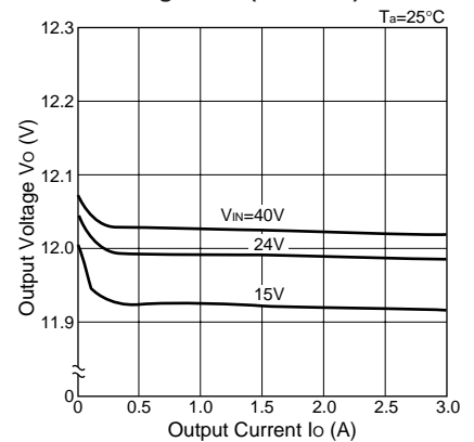
Load Regulation(SI-8120S)
