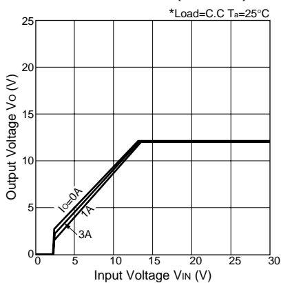
Rise Characteristics(SI-8120S)
