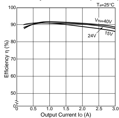
Efficiency Characteristics(SI-8120S)
