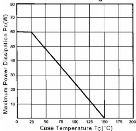
Power Derating
