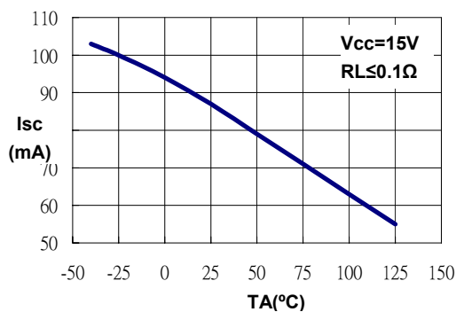
Reference Short Circuit Current vs. Temperature.
