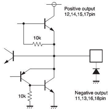
Driver output
