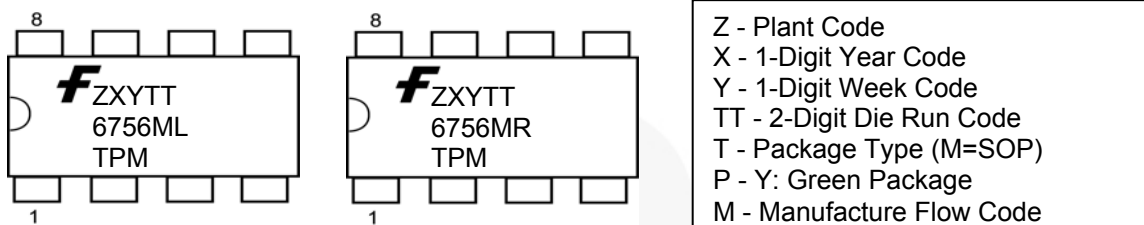
Figure 3. Top Mark
