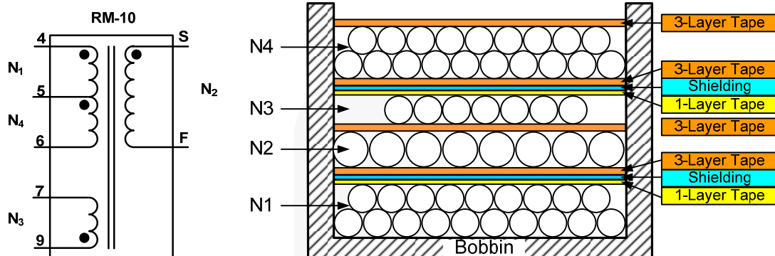
Figure 41. Transformer Specification
