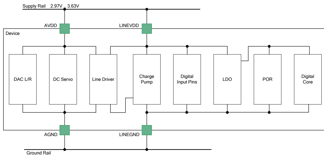
Figure 10 Power Domain Diagram
