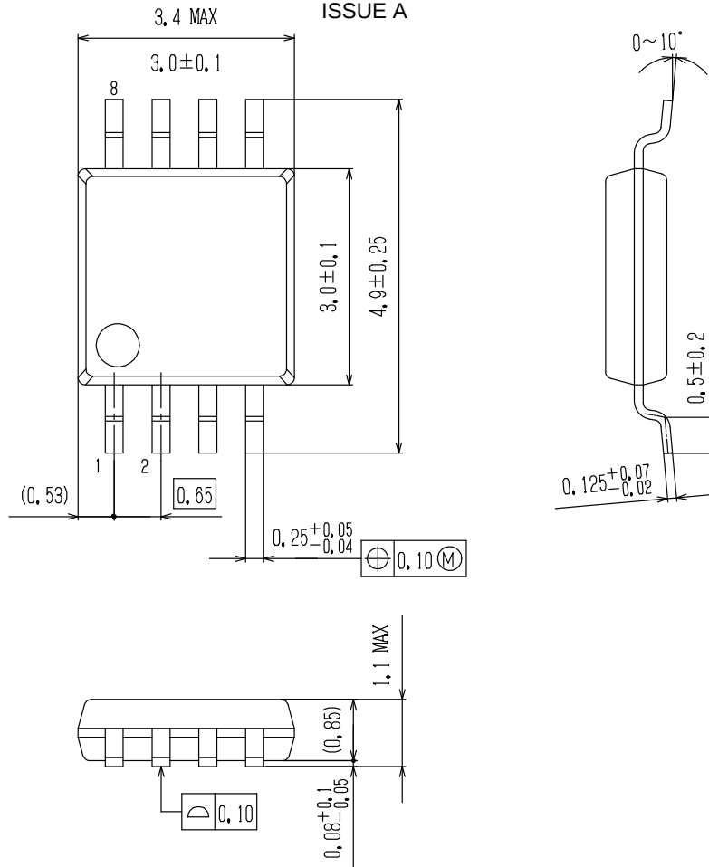
Micro8 / MSOP8 (150 mil) CASE 846AH ISSUE A
