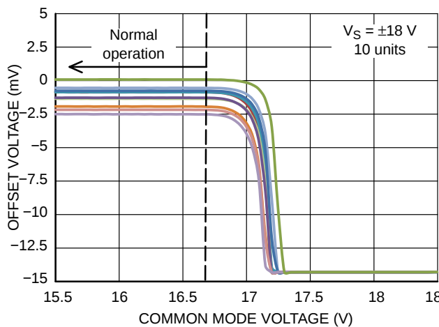
Figure 7. Input Offset Voltage vs. Common Mode Voltage
