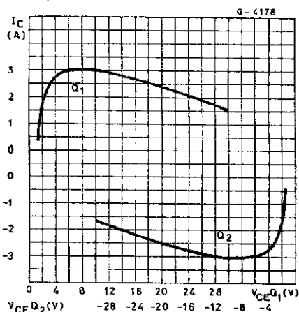
Figure 18 : Maximum Output Current versus Voltage V_{CE}(\text{sat}) across each Output Transistor
