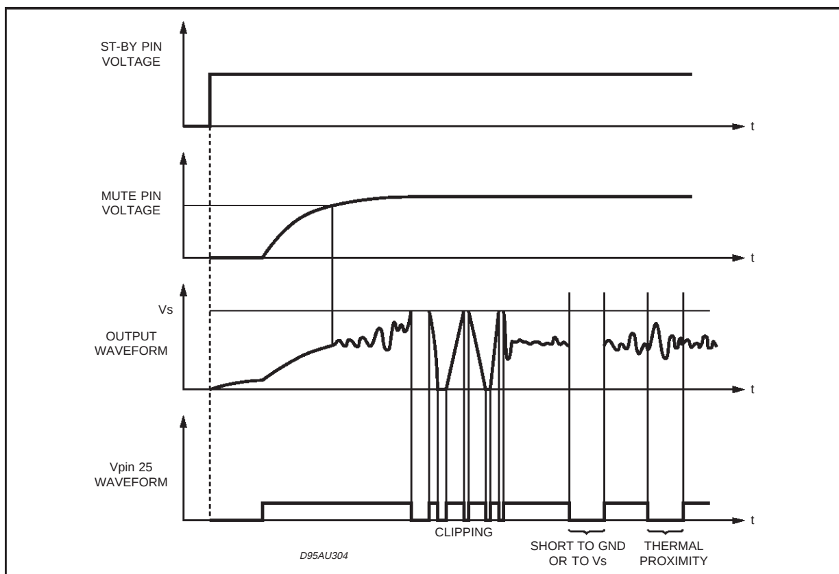
Figure 6: Diagnostics Waveforms.
