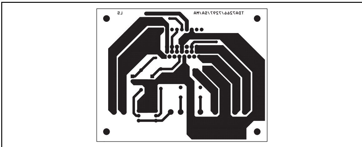
Figure 11. Evaluation Board Bottom Layer Layout
