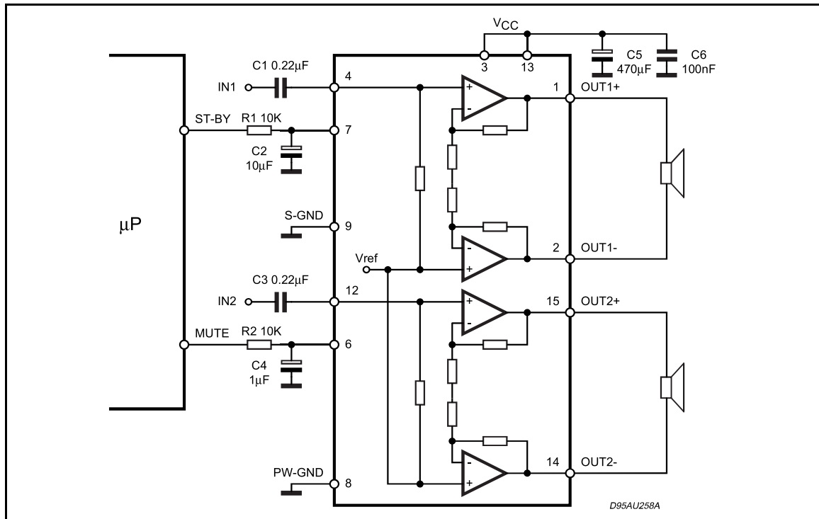
Figure 1. Microprocessor Application
