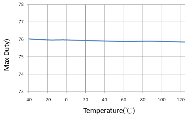
Fig10. Max Duty vs Temperature.
