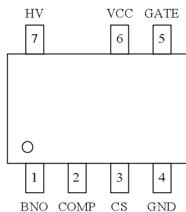
SOP-7 TOP VIEW
