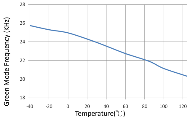
Fig4. Green Mode Frequency vs. Temperature.
