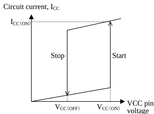
Figure 10-2 Relationship between VCC pin voltage and I_{\text{CC}}
