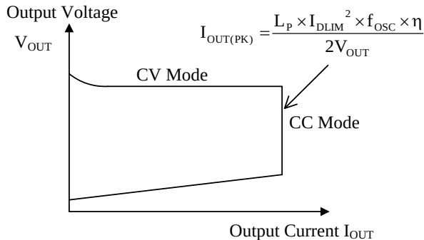
Figure 10-9 CV/CC characteristics
