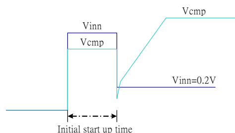
Figure 1. Initial transition response (VDD=5V, V INN = 0.68V, V CMP = 0.53V)
