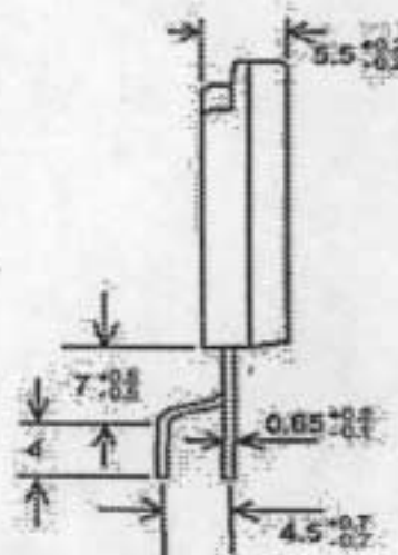
STR-F6600 Series - Outline Drawing
