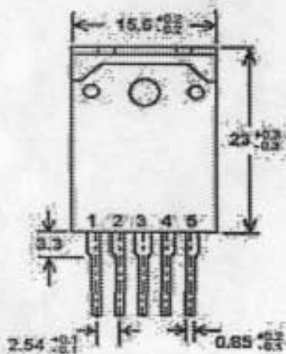
STR-F6600 Series - Outline Drawing
