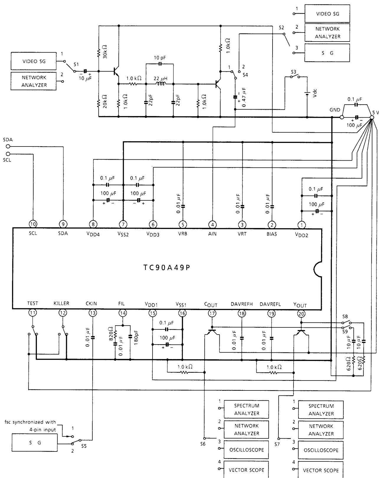
TEST CIRCUIT (TC90A49P)
