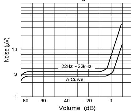
Fig.4 Noise vs. Volume/Gain settings
