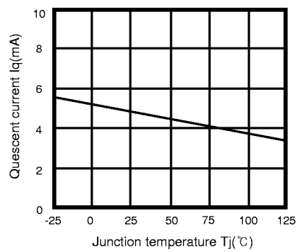
FIG.5 Quiescent Current vs. Temperature( T_j )
