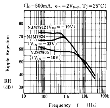
NJM7905/15/24 Ripple Rejection vs. Frequency
