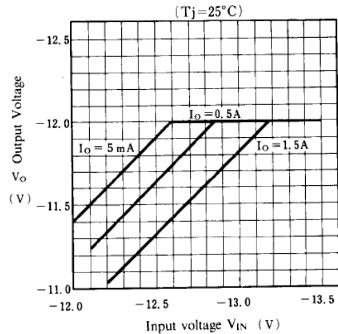
NJM7912 Output Voltage vs. Low Input Voltage
