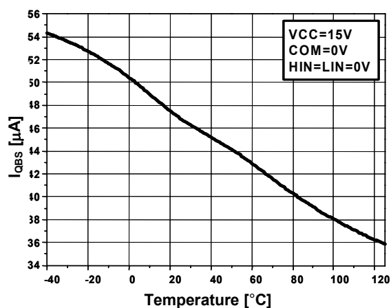
Figure 23. I_{QBS} vs. Temp.
