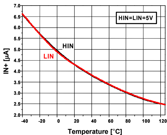
Figure 29. Input Bias Current vs. Temp.
