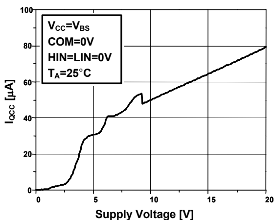
Figure 20. I_{QCC} vs. Supply Voltage
