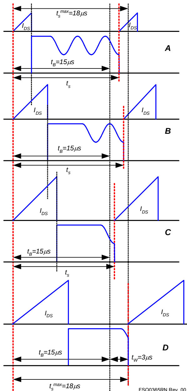
Figure 27. QRC Operation with Limited Frequency
