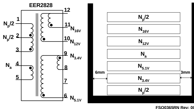
Figure 30. Transformer Schematic Diagram
