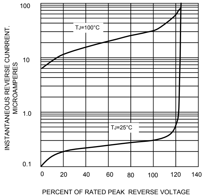
FIG.4-TYPICAL REVERSE CHARACTERISTICS
