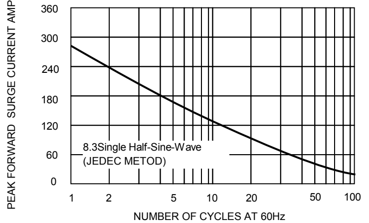
FIG.2-MAXIMUM NON-REPETITIVE SURGE
