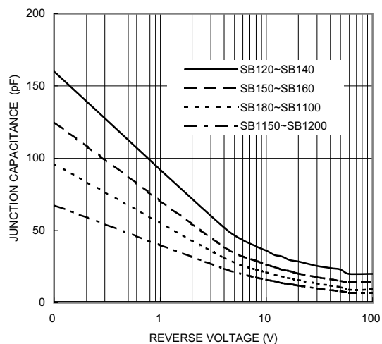
FIG. 5-TYPICAL JUNCTION CAPACITANCE
