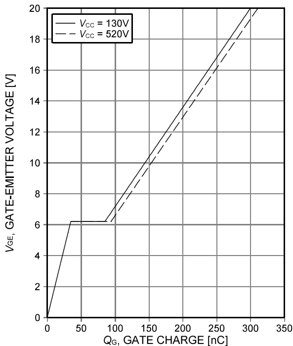
Figure 15. Typical gate charge ( I_C=50\text{A} )
