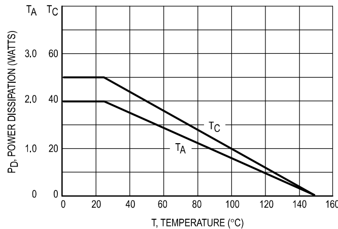
Figure 1. Power Derating
