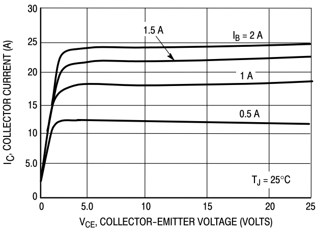
Figure 7. Typical Output Characteristics
