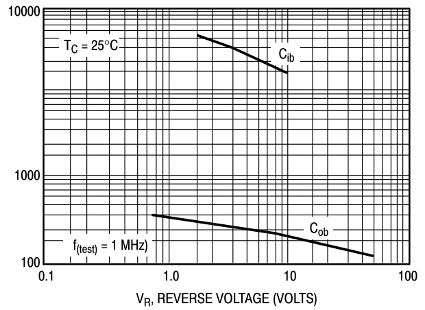
Figure 15. MJL21194 Typical Capacitance
