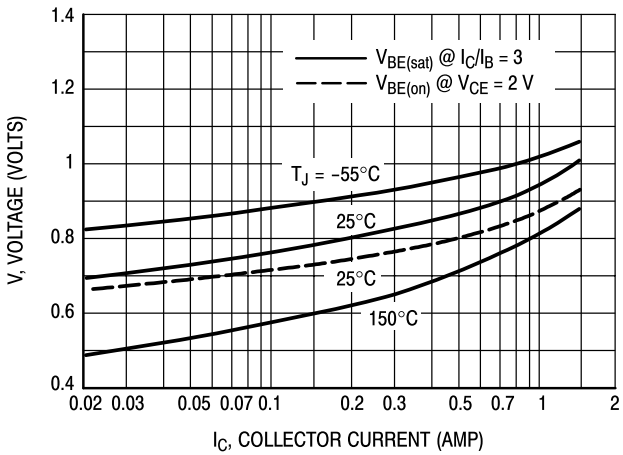
Figure 3. Base-Emitter Voltage
