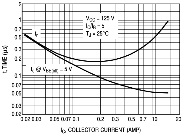
Figure 8. Turn-On Time
