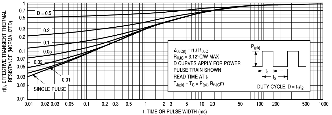
Figure 10. Thermal Response
