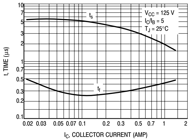
Figure 9. Turn-Off Time
