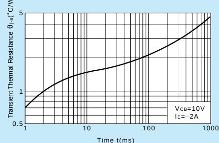
\theta_{j-a}-t Characteristics
