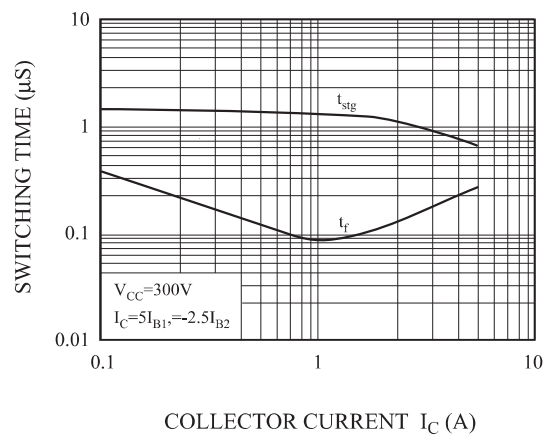
Fig 6. SWITCHING CHARACTERISTIC
