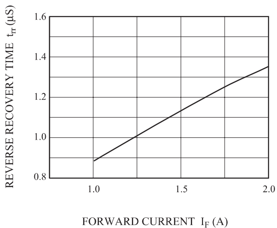
Fig 7. t_{rr} - I_F
