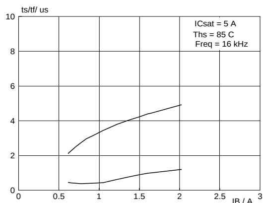
Fig.9. Typical collector storage and fall time. I_{C\ sat} = 5\ A; T_j = 85^\circ C; f = 16\ kHz
