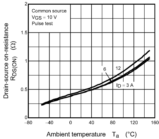
Fig. 8.7 R_{DS(ON)} - T_a
