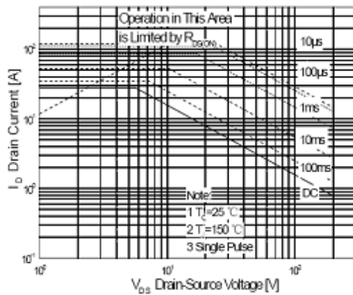
Maximum Safe Operating Area For JCS650C/S
