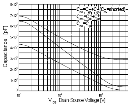
Capacitance Characteristics
