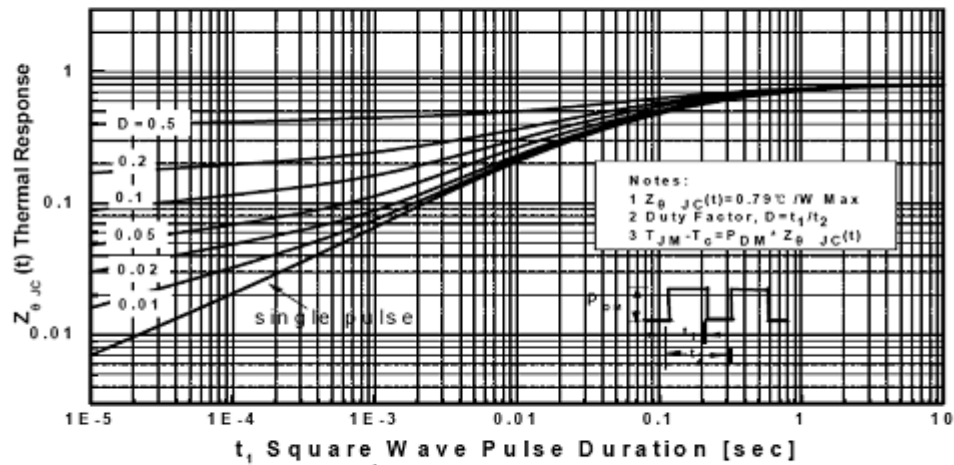
Transient Thermal Response Curve For JCS650F
