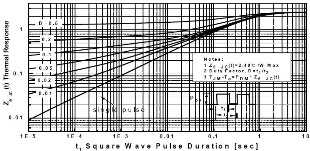
Transient Thermal Response Curve For JCS650F
