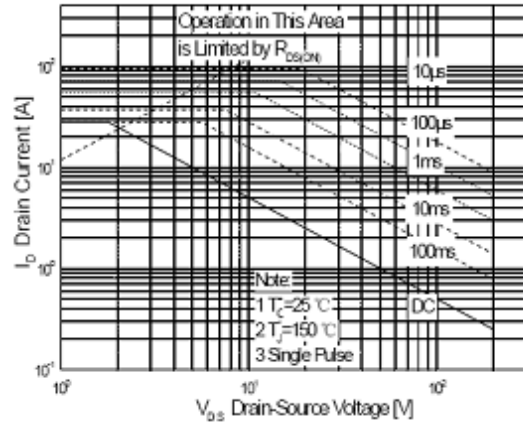
Maximum Safe Operating Area For JCS650F
