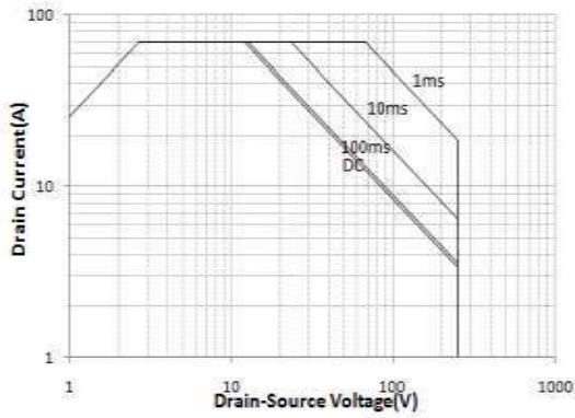
Maximum safe operating area For JCS86N25WT/ABT
