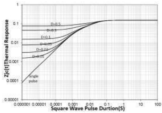
Transient Thermal Response Curve For JCS86N25GCT
