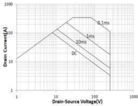
Maximum safe operating area For JCS86N25GCT
