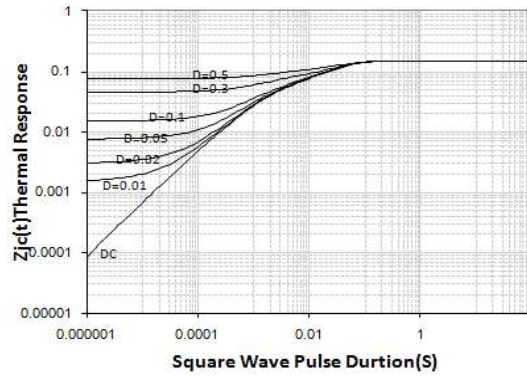
Transient Thermal Response Curve For JCS86N25GCT
