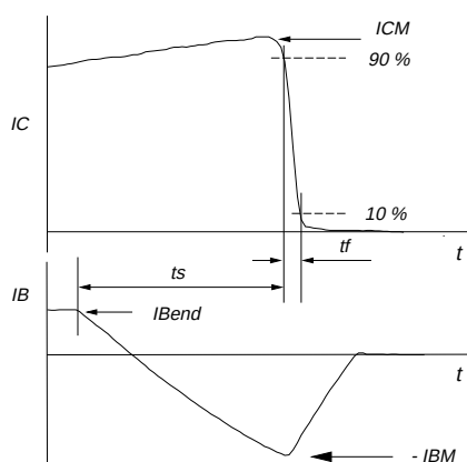
Fig.2. Switching times definitions.
